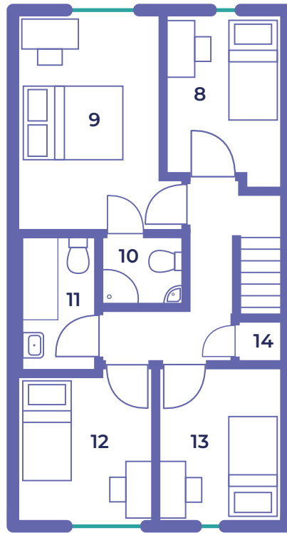
House type C ground floor
